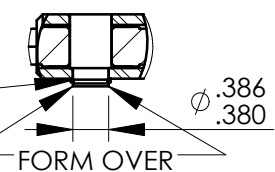
DETAIL A SCALE 1 : 2 DEFORM BEFORE CALIBRATION
