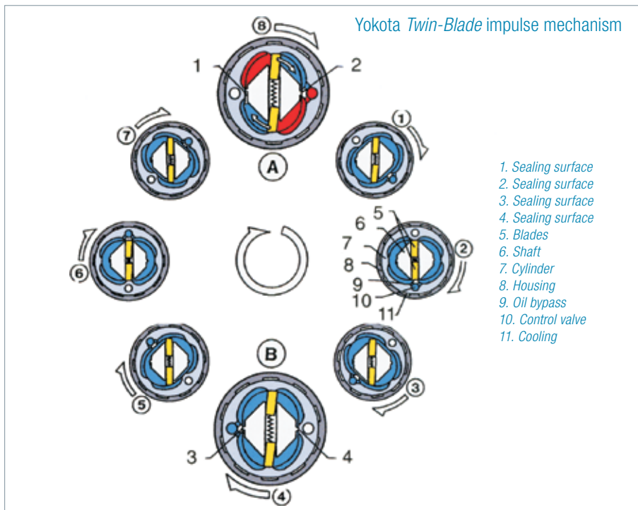
Double chamber air motor principle
