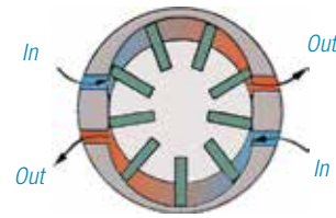
Double Chamber Air Motor
