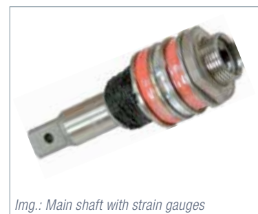
Img.: Main shaft with strain gauges
