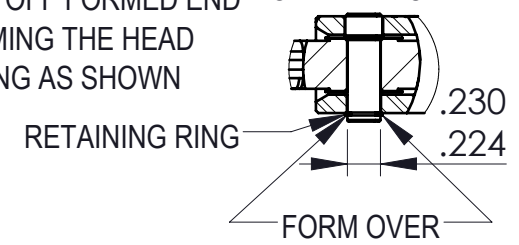
DETAIL A SCALE 4 : 5 DEFORM BEFORE CALIBRATION
